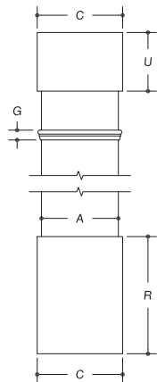
Fig. 1 Standard Cap & Base
