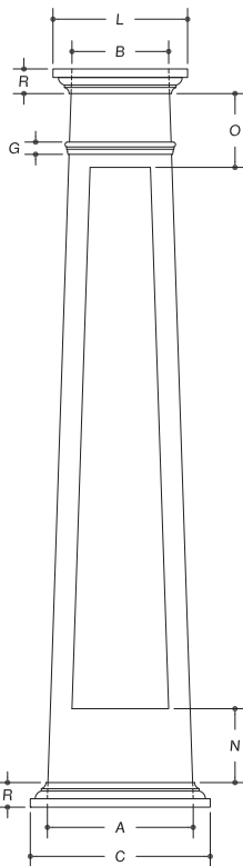
Fig. 3 Craftsman with Traditional Cap & Base
