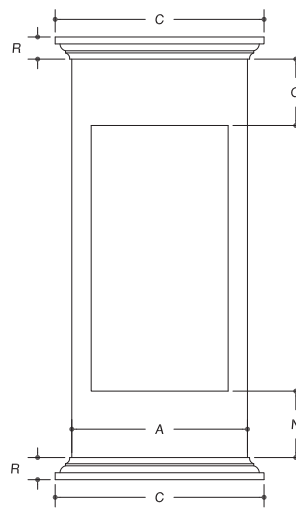
Fig. 4 Pedestal with Traditional Cap & Base
